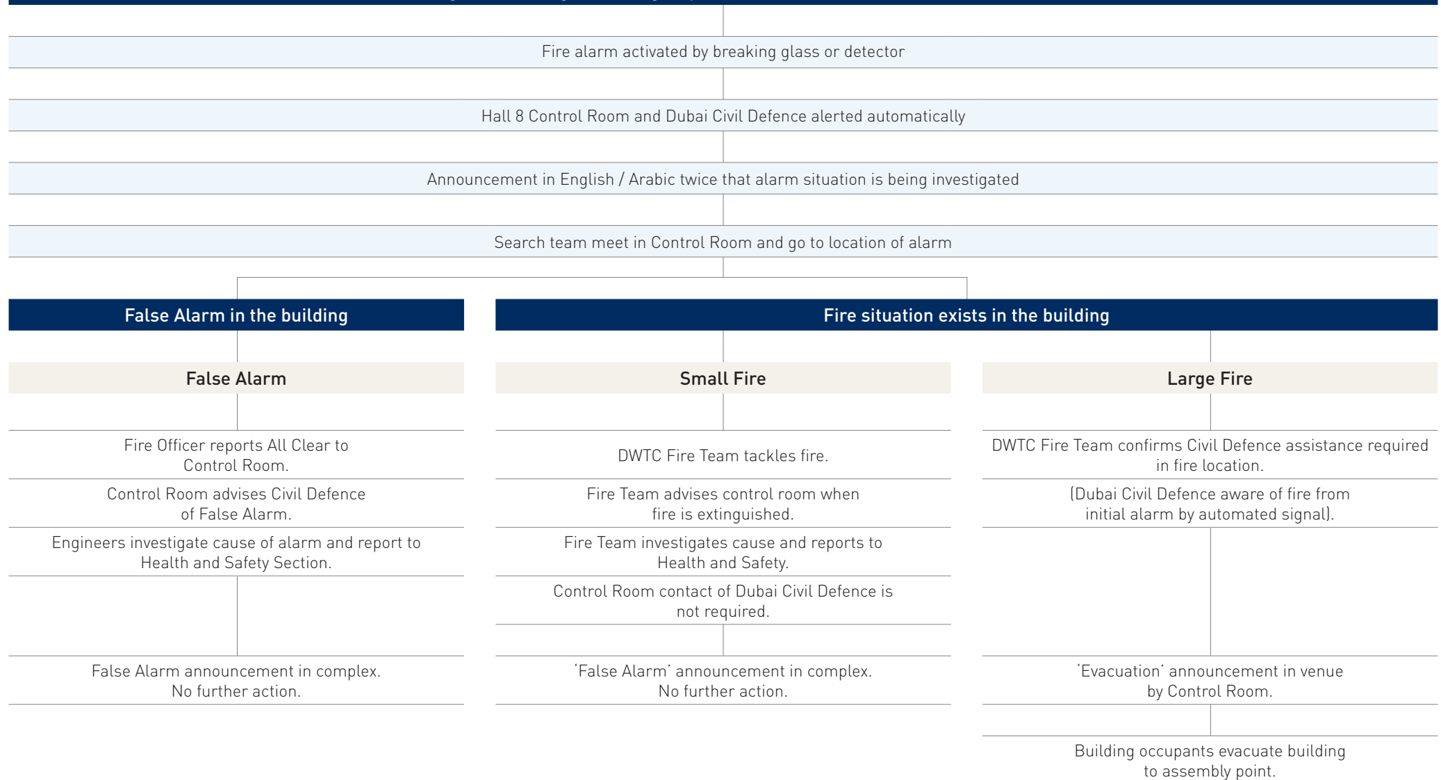
Flow diagram detailing the Emergency Procedure for the Dubai World Trade Centre
