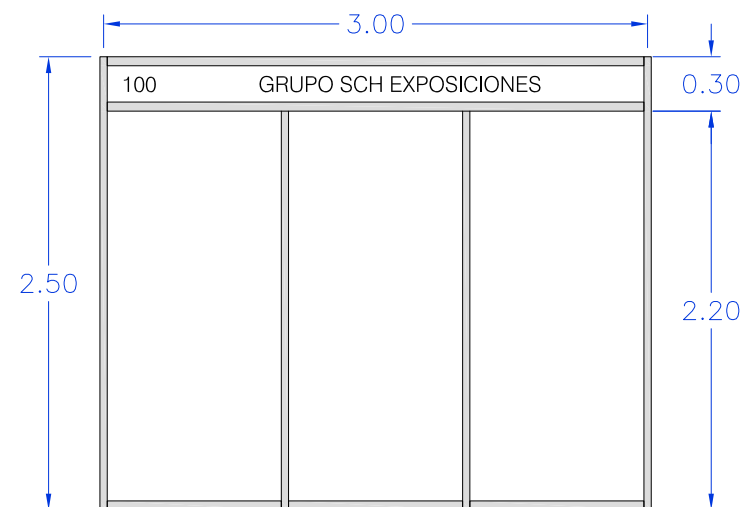
Vista frontal
